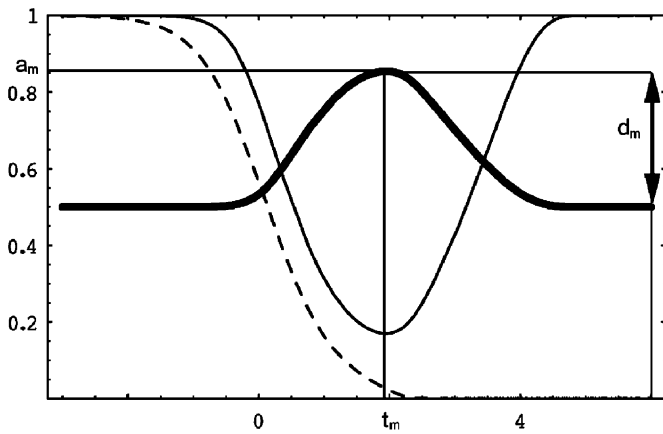
Fig. 5. Time response of the GAL pathway depicted in Fig. 2A. The initial state consists of 0.1 unit of Gal4p/DNA (bold line), and 1 unit of Gal80p (plain line). Two units of galactose (dashed line) are initially introduced, unless otherwise stated. Note the log scale on the time axis. Along the ordinate axis, the Gal4p scale has been amplified five-fold, and the galactose scale has been decreased two-fold. This simulation involves no delay in transformations. In this respect, the result may be compared with Fig. 4A.
